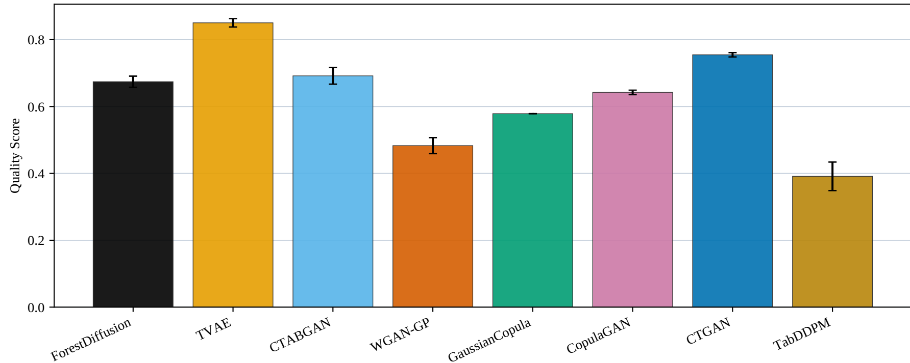
Metro Interstate — Quality Score (mean \pm SD, 10 seeds)
